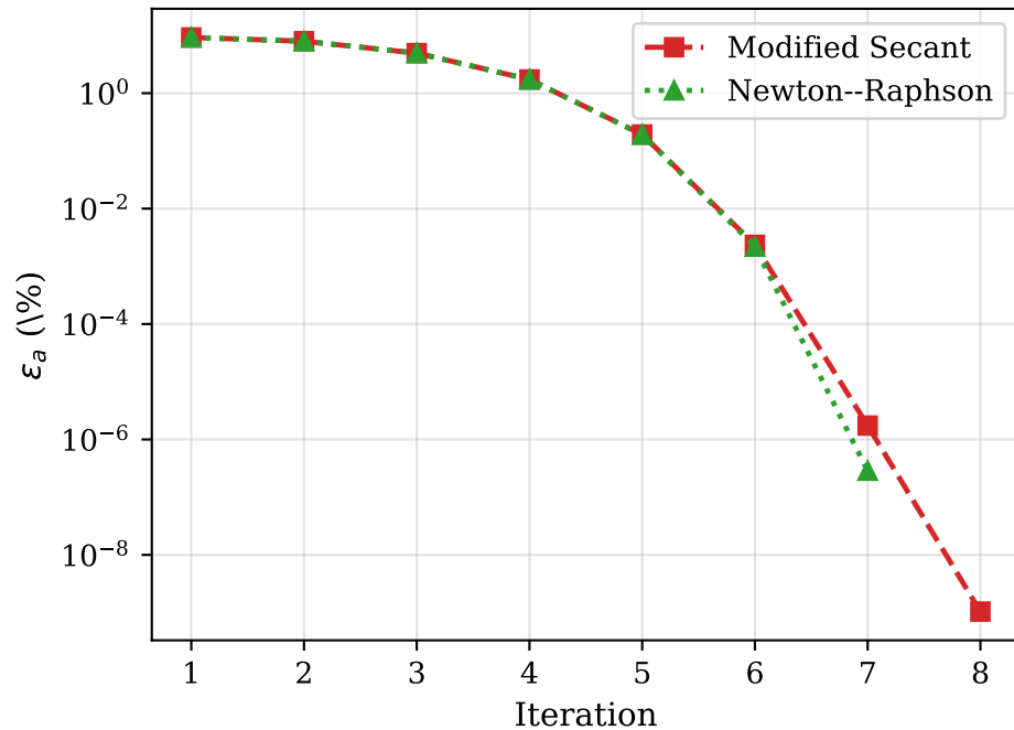
Modified Secant vs N-R Root 2 ( \theta^* = 51.53^\circ )
