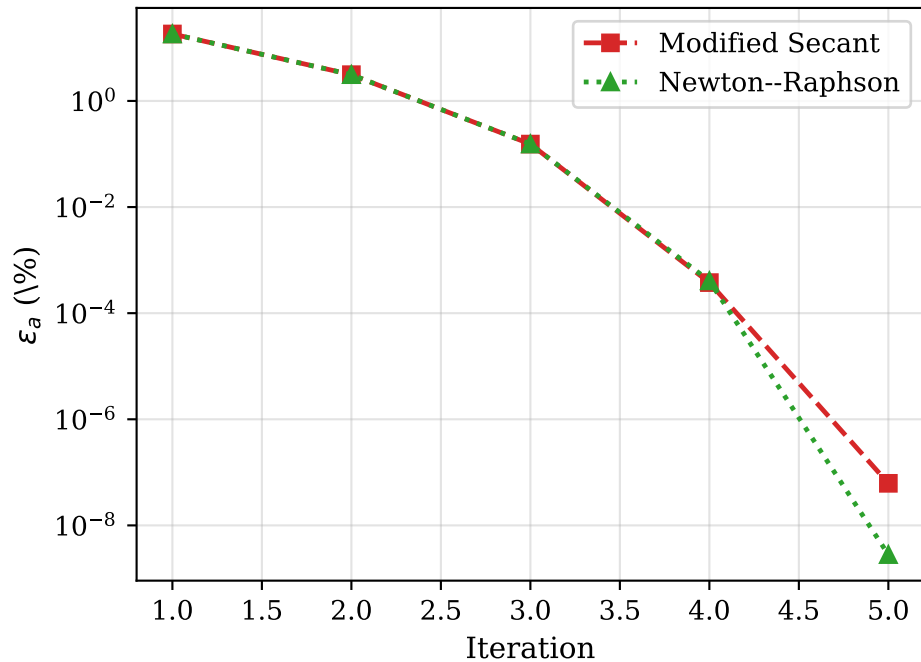
Modified Secant vs N-R Root 1 ( \theta^* = 37.96^\circ )
