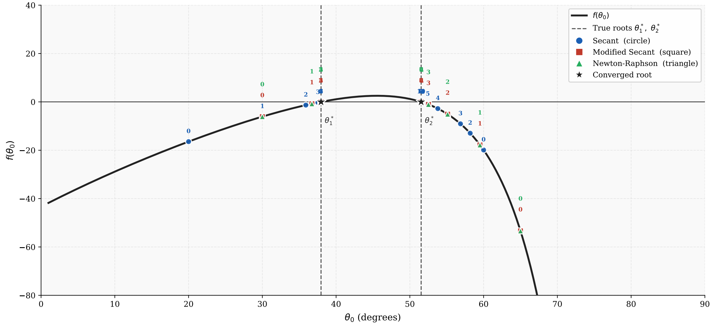
Successive Iterates of All Three Methods Converging to Both Roots on f(\theta_0)
