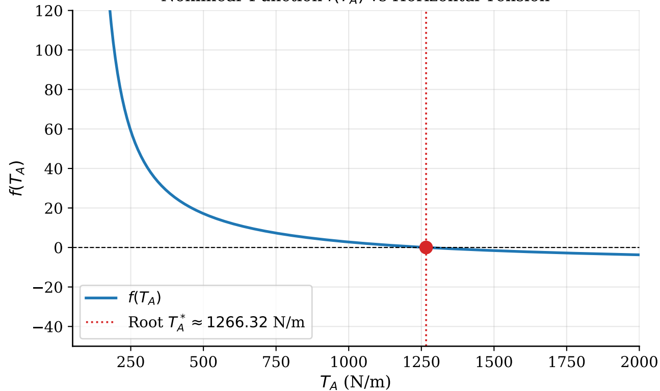
Nonlinear Function f(T_A) vs Horizontal Tension
