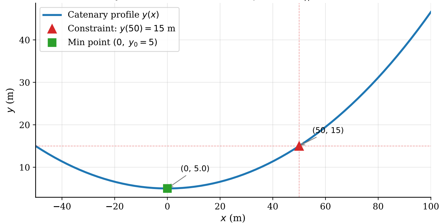
Catenary Cable Profile ( w = 10 \text{ N/m} , y_0 = 5 \text{ m} , T_A^* \approx 1266.32 \text{ N/m} )
