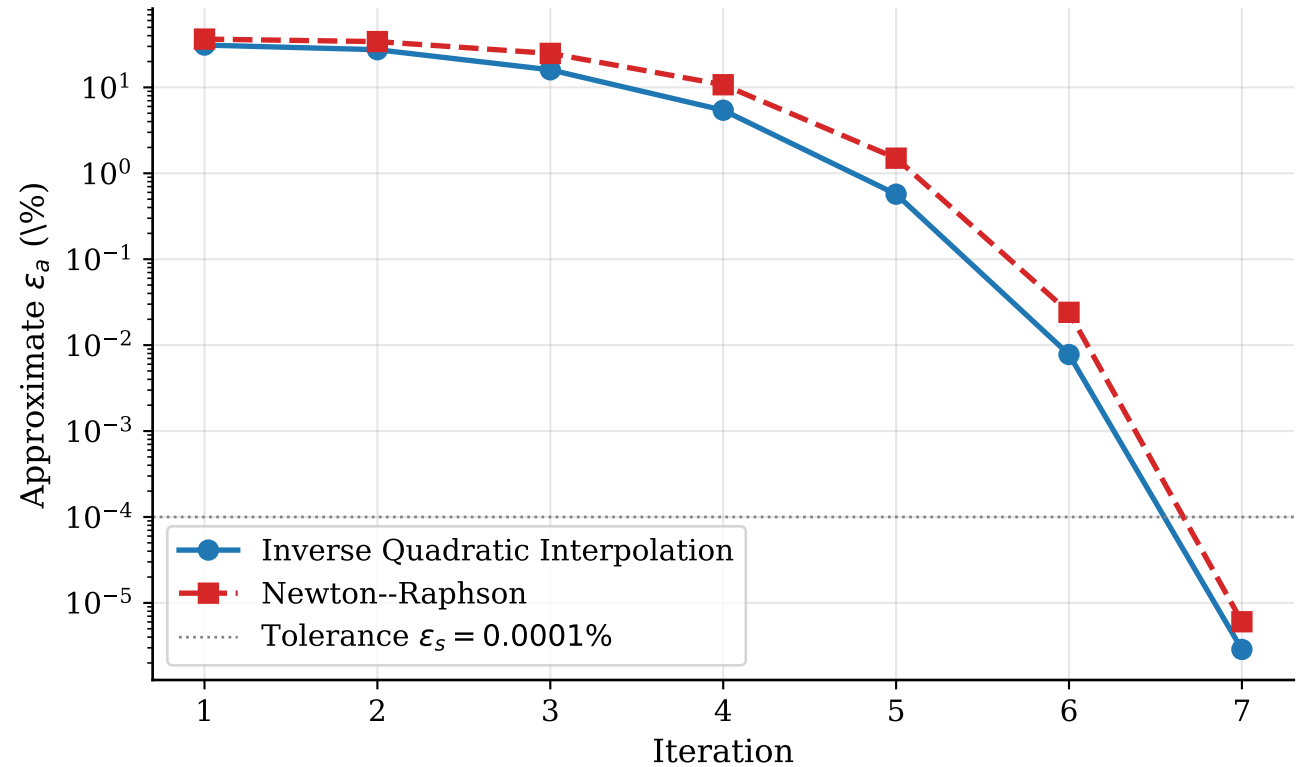
Error Convergence: IQI vs Newton--Raphson
