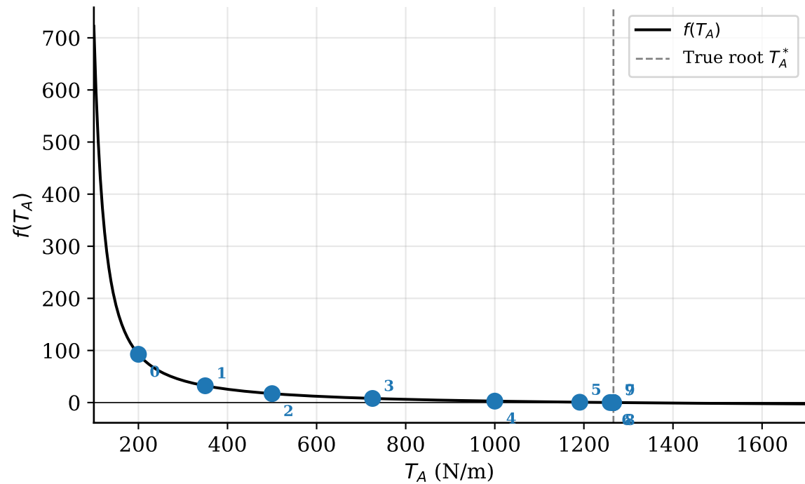
Successive Iterates - IQI
