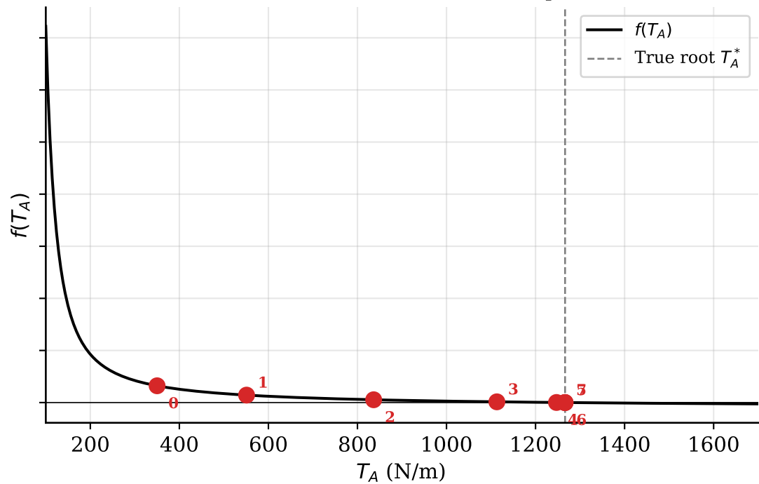
Successive Iterates - Newton--Raphson
