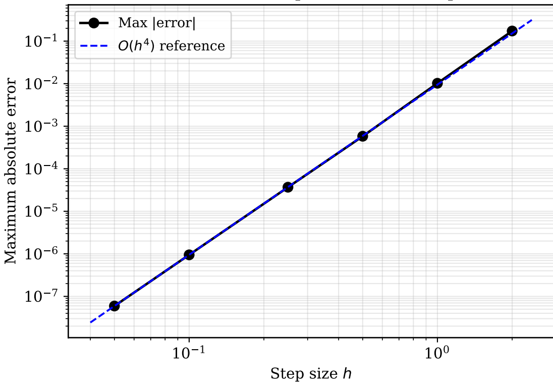
RK4 Global Error vs Step Size (fitted slope = 4.03)
