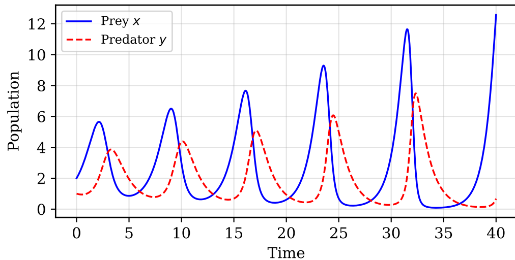
(a) Euler — Time Domain
