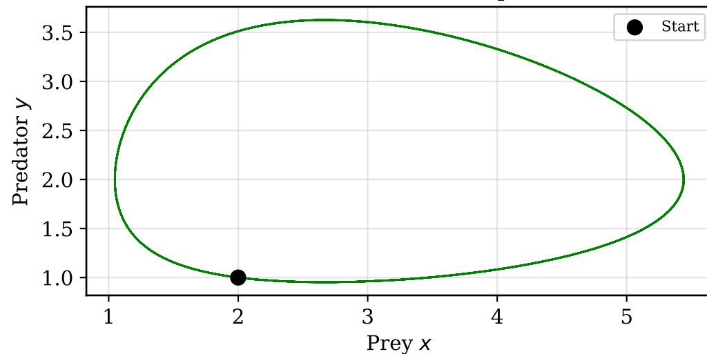
(d) RK4 — Phase Plane (closed orbit, Hamiltonian preserved)
