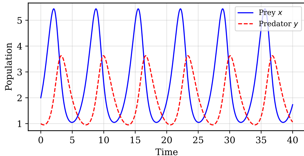
(c) RK4 — Time Domain
