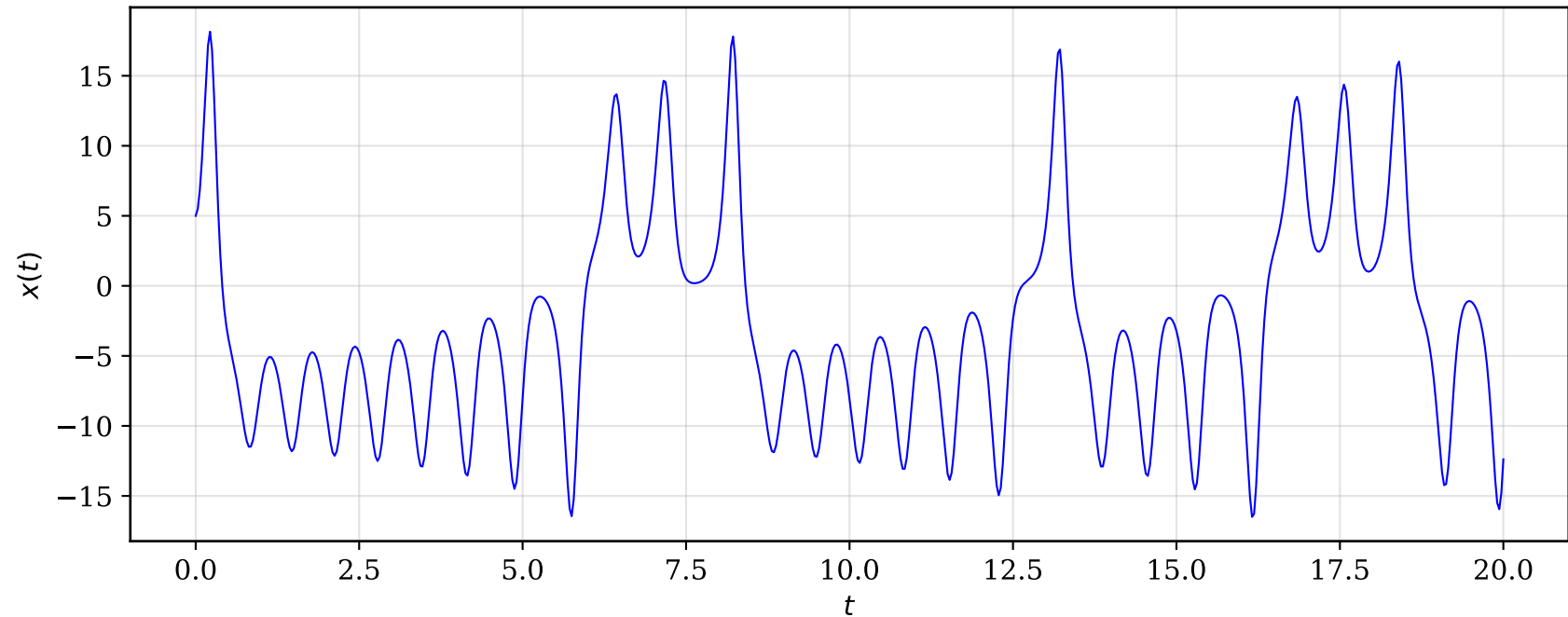
Lorenz System: x(t) vs t ( \sigma = 10 , b = 8/3 , r = 28 , IC = (5, 5, 5))
