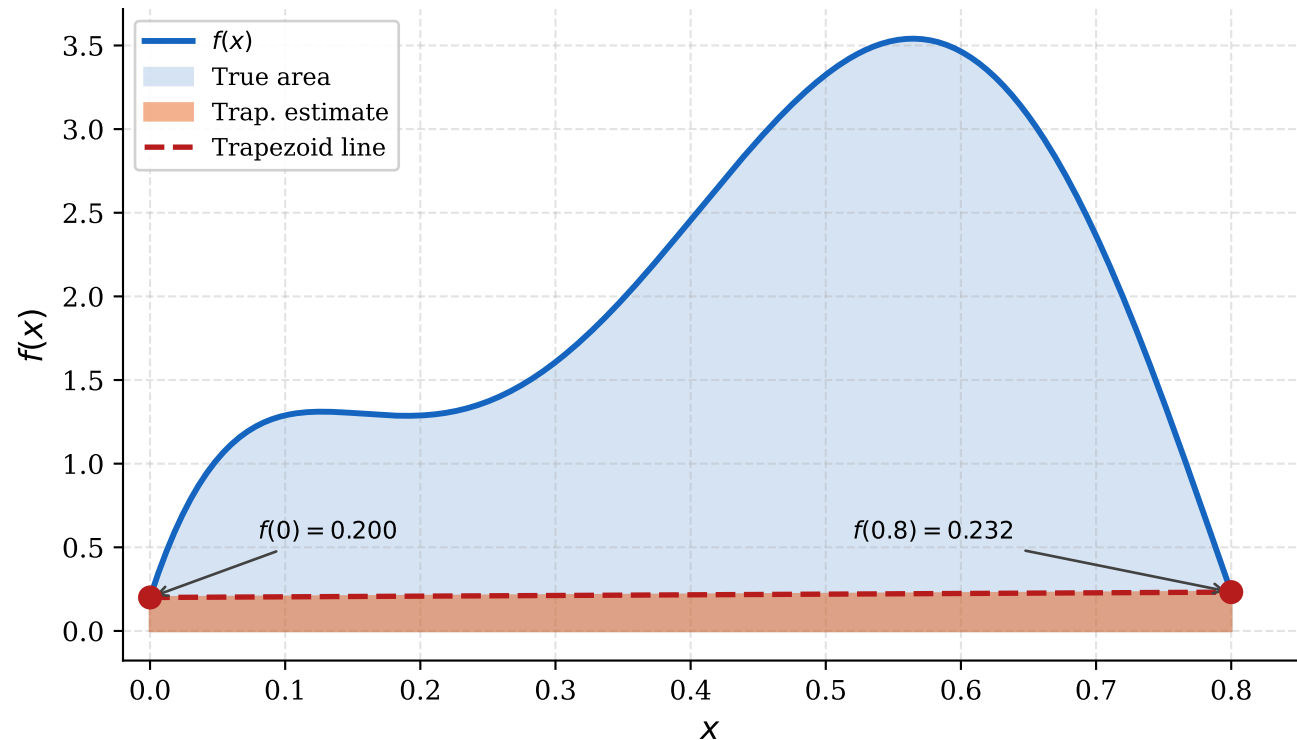
Example 19.1—Single Trapezoidal Rule I = 0.1728 | Exact = 1.6405 | \varepsilon_t = 89.5\%
