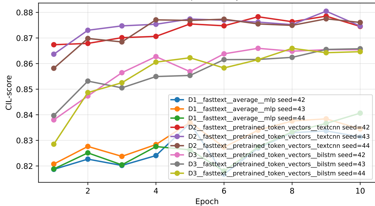
DNN epoch analysis
