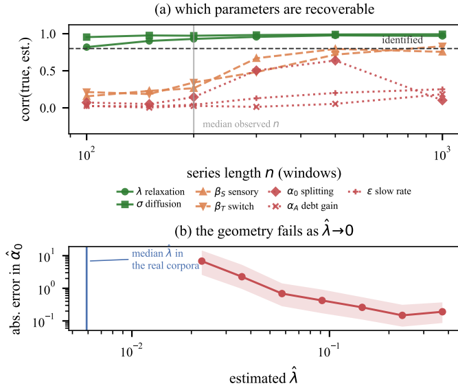
Fig. 2: (a) Rank recovery against series length, 2000 replicates per point. (b) The mechanism: error in the recovered splitting factor rises as \hat{\lambda} falls, because a = \theta_2/\theta_1 . The median \hat{\lambda} in the real corpora lies below the whole simulated range.
