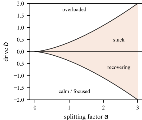
(b) bifurcation set
