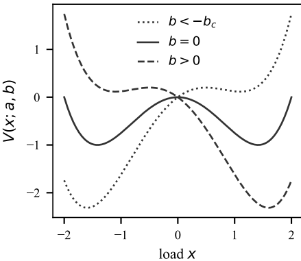
(a) cusp potential
