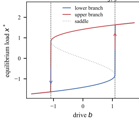
(c) hysteresis, width \Delta b = \frac{4}{3\sqrt{3}}a^{3/2}
