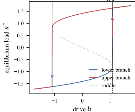
(c) hysteresis, width \Delta b = \frac{4}{3\sqrt{3}}a^{3/2}
