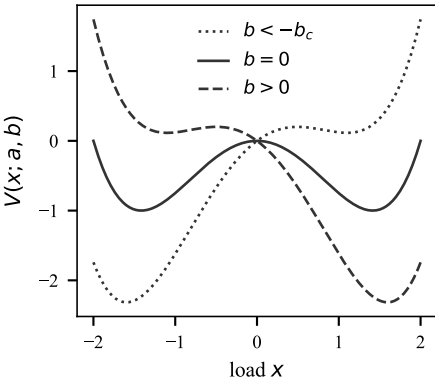
(a) cusp potential
