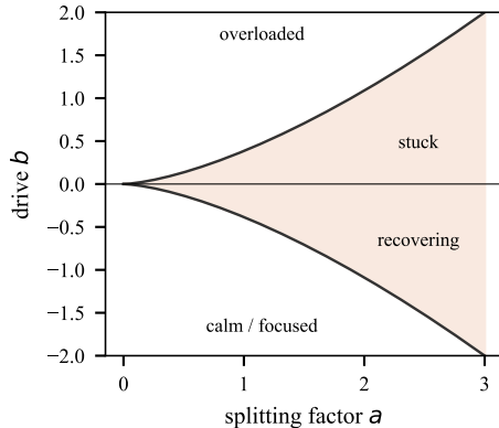
(b) bifurcation set
