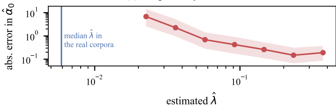
(b) the geometry fails as \hat{\lambda} \rightarrow 0
