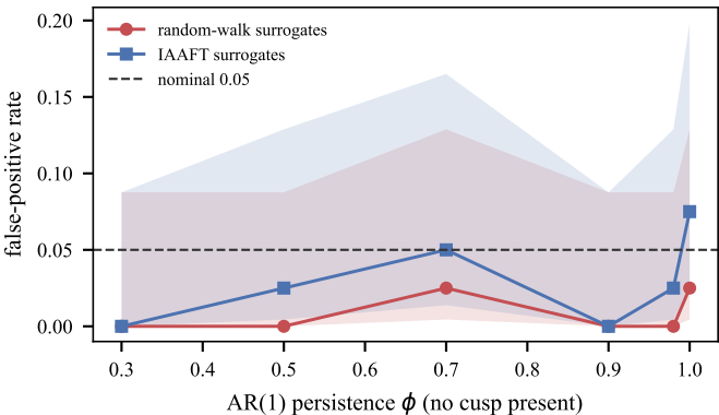
calibrated size vs persistence (40 reps/point)
