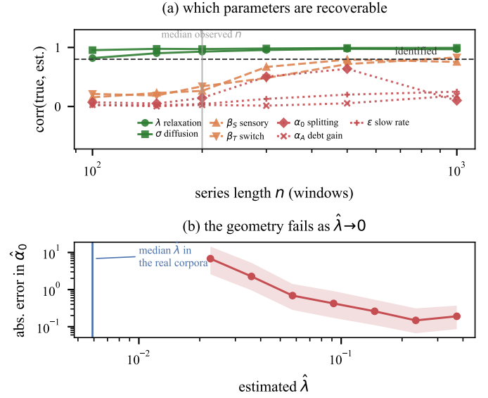
Fig. 2. (a) Recovery correlation against series length, 600 replicates per point. Only \lambda and \sigma clear a useful threshold at the median observed length. (b) The failure mechanism: absolute error in the recovered splitting factor rises as \hat{\lambda} falls, because a = \theta_2/\theta_1 . The median \hat{\lambda} in the real corpora lies below the whole simulated range.
