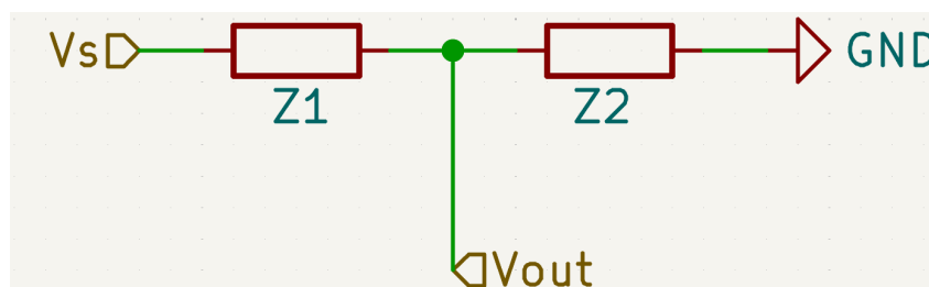
Figure 2.1: Voltage divider circuit with two resistive components, V_s is the supply voltage and V_{out} is the reduced voltage reference.
