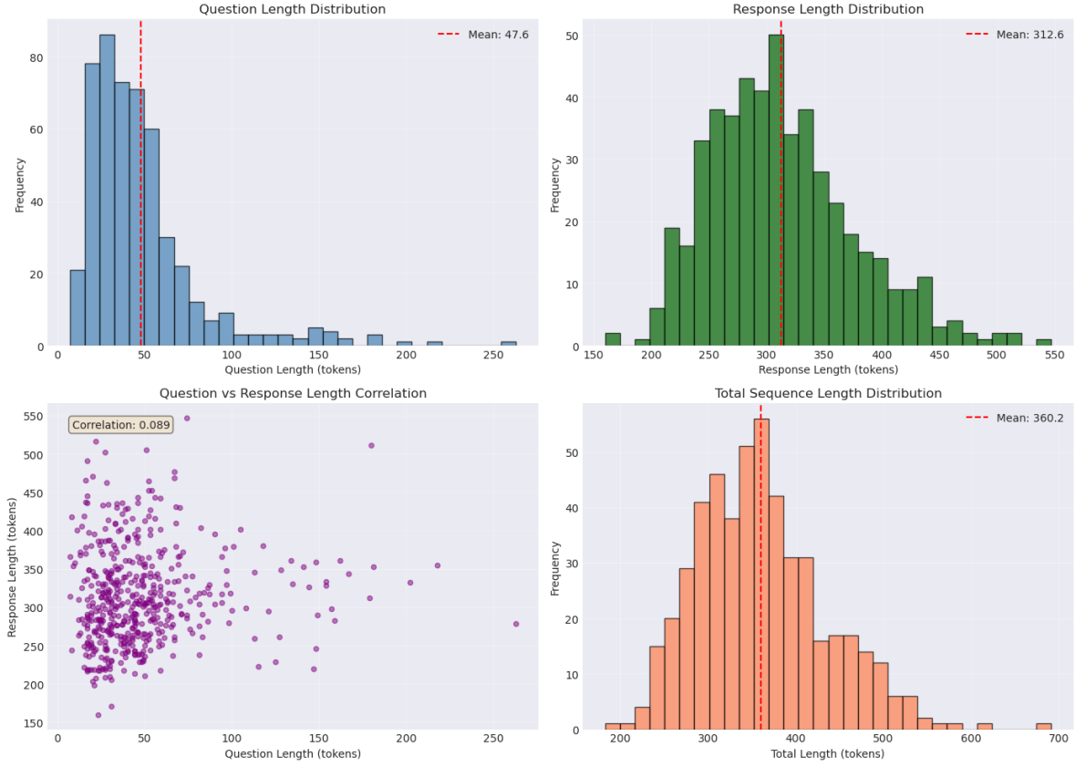
Figure 5: Dataset characteristics. Mean question length 47.6 tokens (95th percentile 115.1), mean response length 312.6 (95th percentile 431.1), mean total 360.2 tokens. Question–response length correlation is weak.
