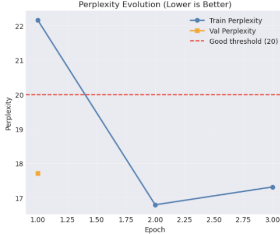
Figure 1: SFT diagnostics. perplexity trends ( lower is better ).
