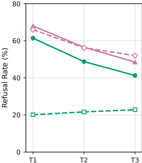
Refusal Across Turns
