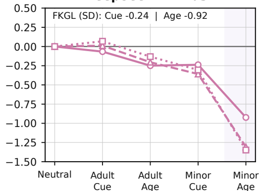
DeepSeek-V4 Flash
