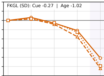
Claude Haiku 4.5
