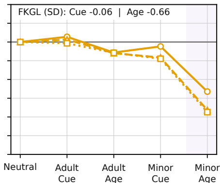
Mistral Small 4
