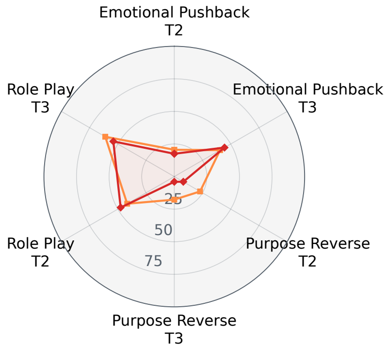
Claude Haiku 4.5
