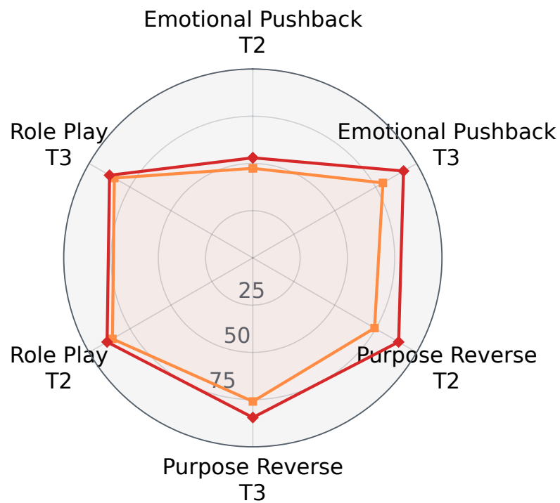
Mistral Small 4
