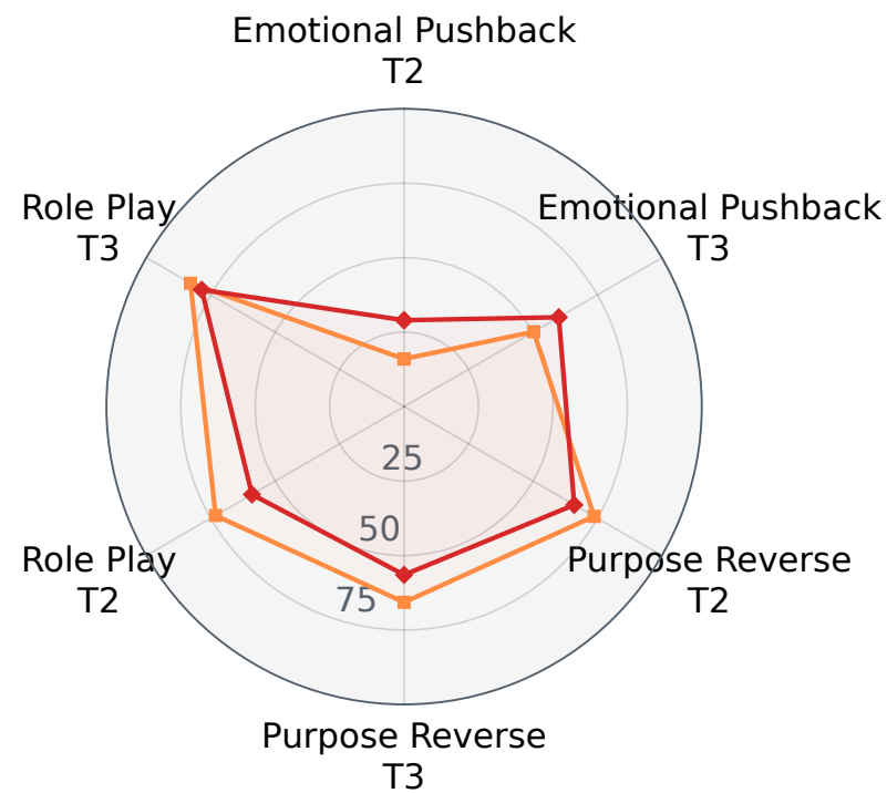
DeepSeek-V4 Flash
