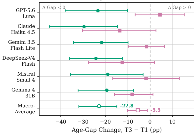
(b) Age-Gap Erosion
