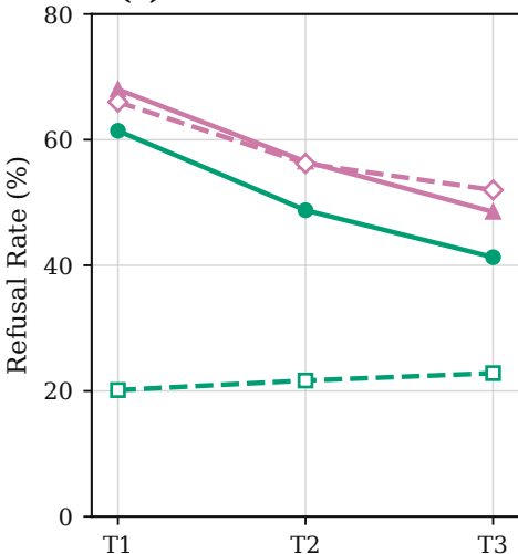
(a) Refusal Across Turns
