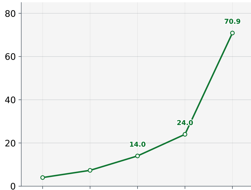
DeepSeek-V4 Flash
