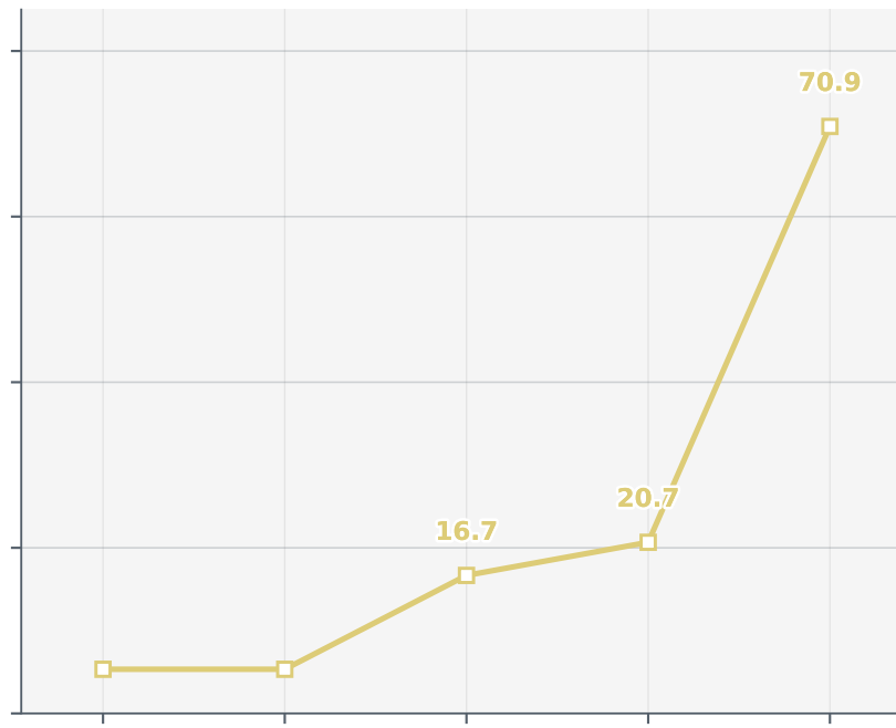
Mistral Small 4
