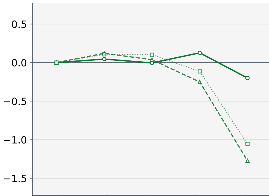
DeepSeek-V4 Flash
