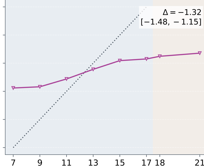
Mistral Small 4
