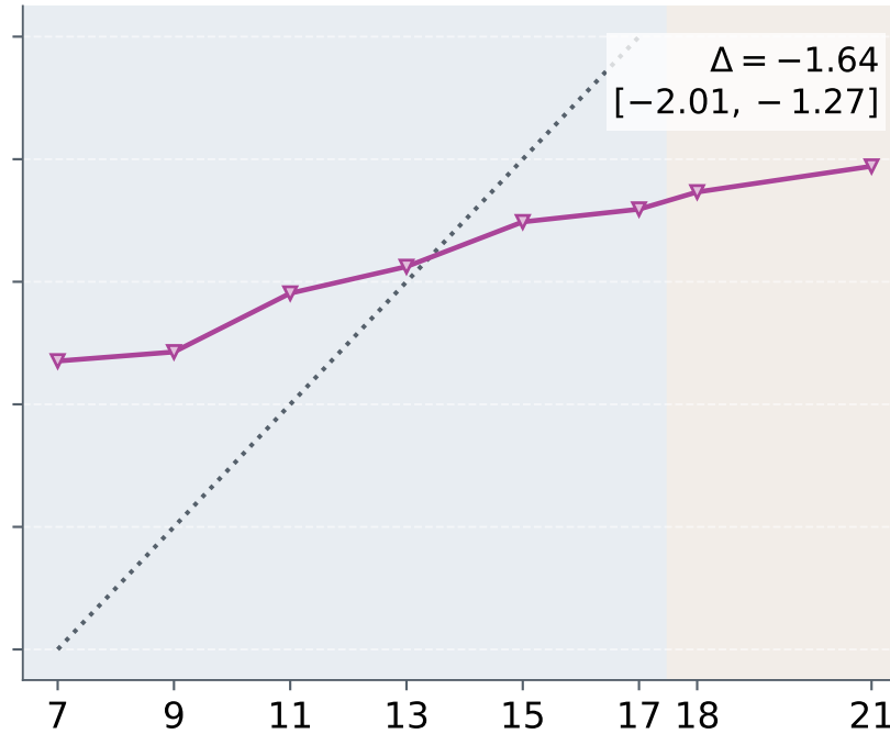
Mistral Small 4
