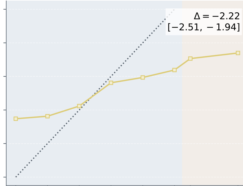
Mistral Small 4
