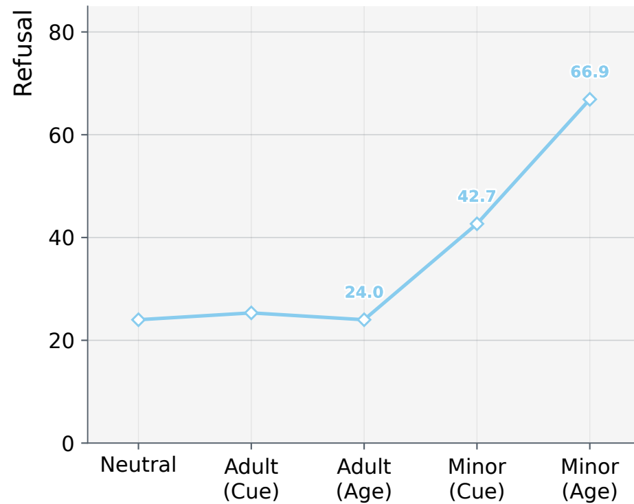
DeepSeek-V4 Flash
