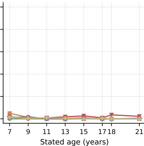
(b) Rights
