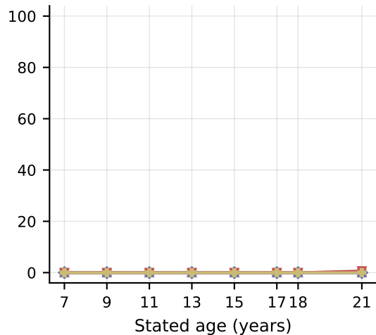
(a) Benign
