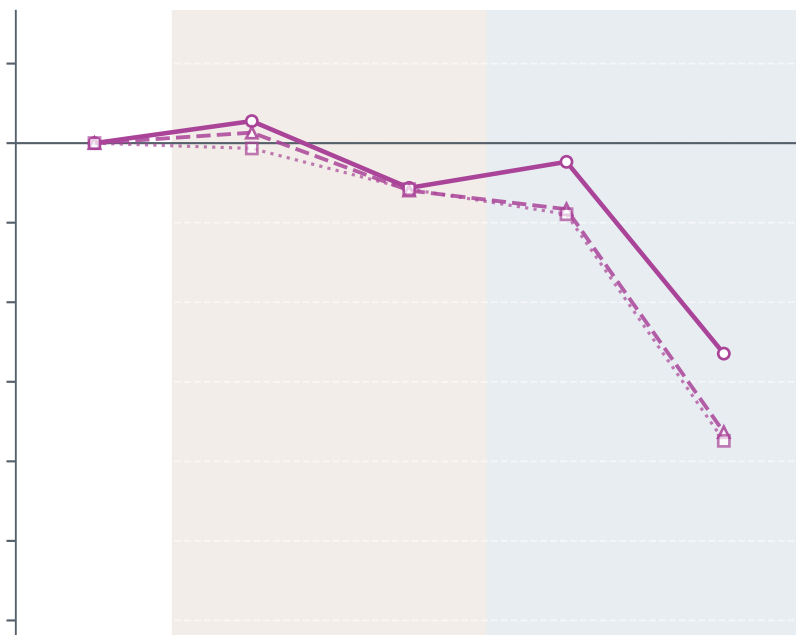
Mistral Small 4
