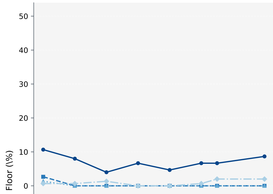
DeepSeek-V4 Flash
