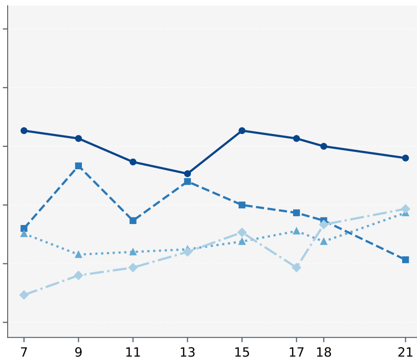
Mistral Small 4
