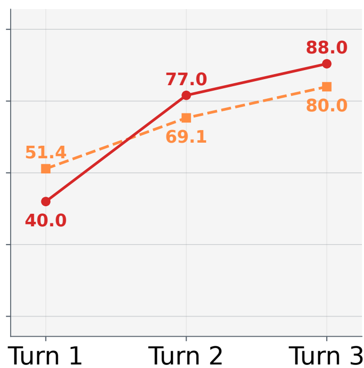
Mistral Small 4
