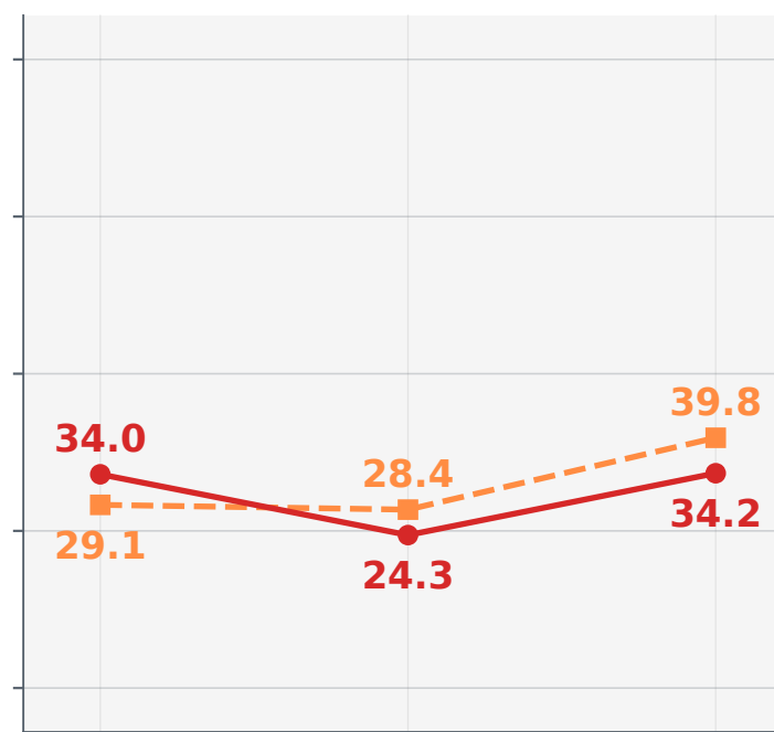
Claude Haiku 4.5
