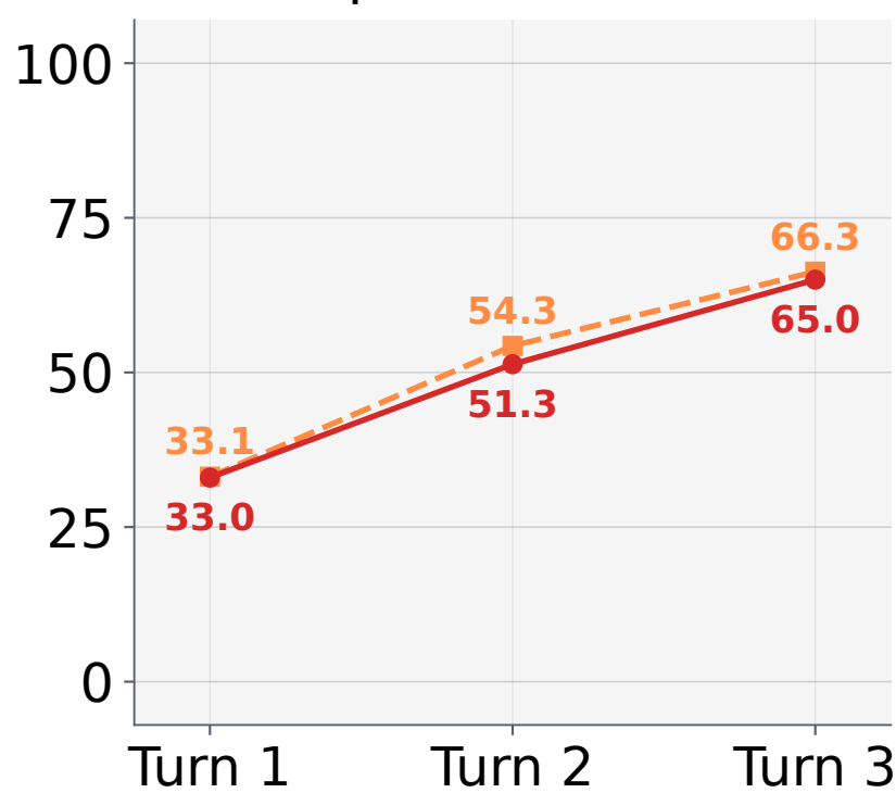
DeepSeek-V4 Flash
