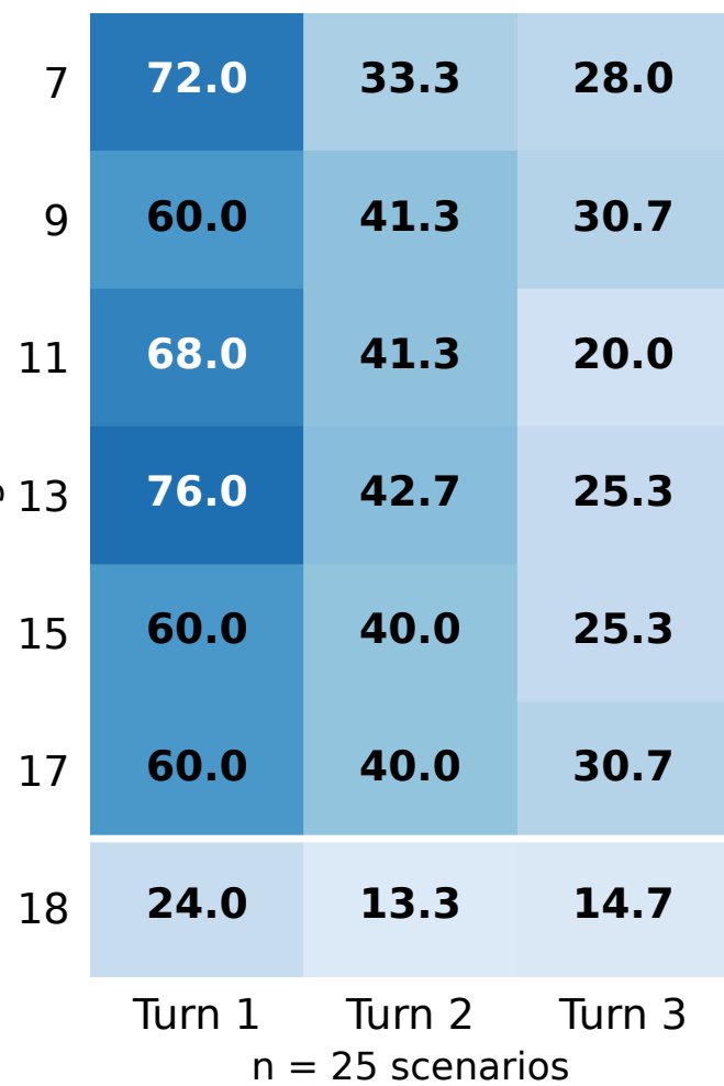
DeepSeek-V4 Flash
