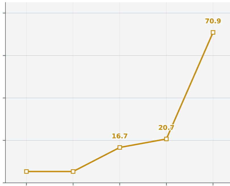
Mistral Small 4
