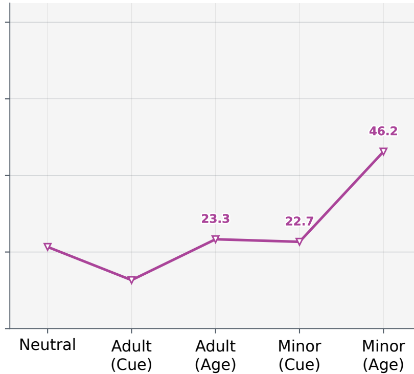
Mistral Small 4
