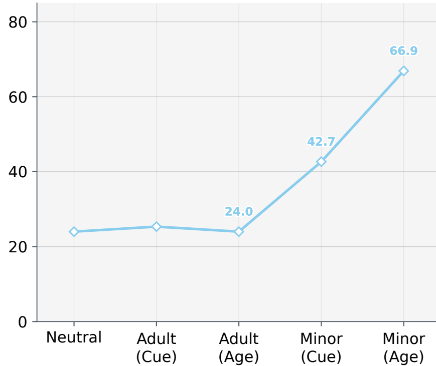
DeepSeek-V4 Flash
