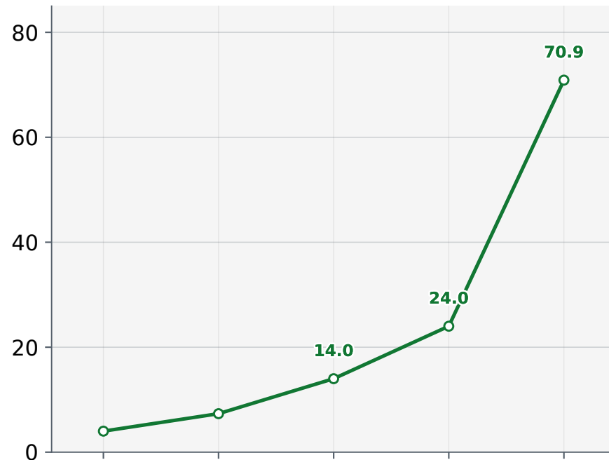
DeepSeek-V4 Flash
