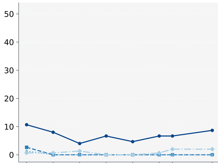
DeepSeek-V4 Flash
