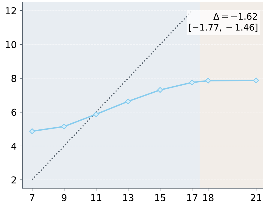
DeepSeek-V4 Flash
