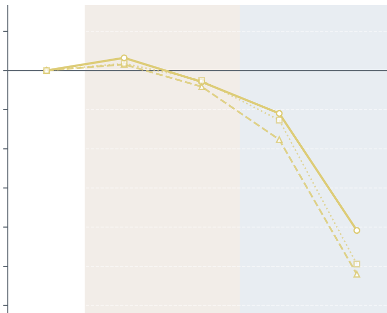
Claude Haiku 4.5
