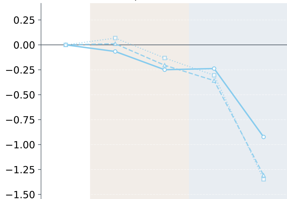
DeepSeek-V4 Flash
