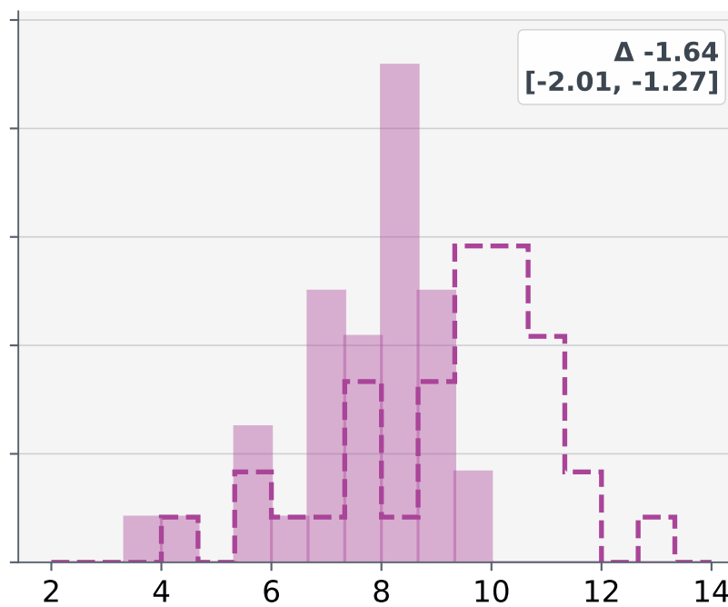
Mistral Small 4
