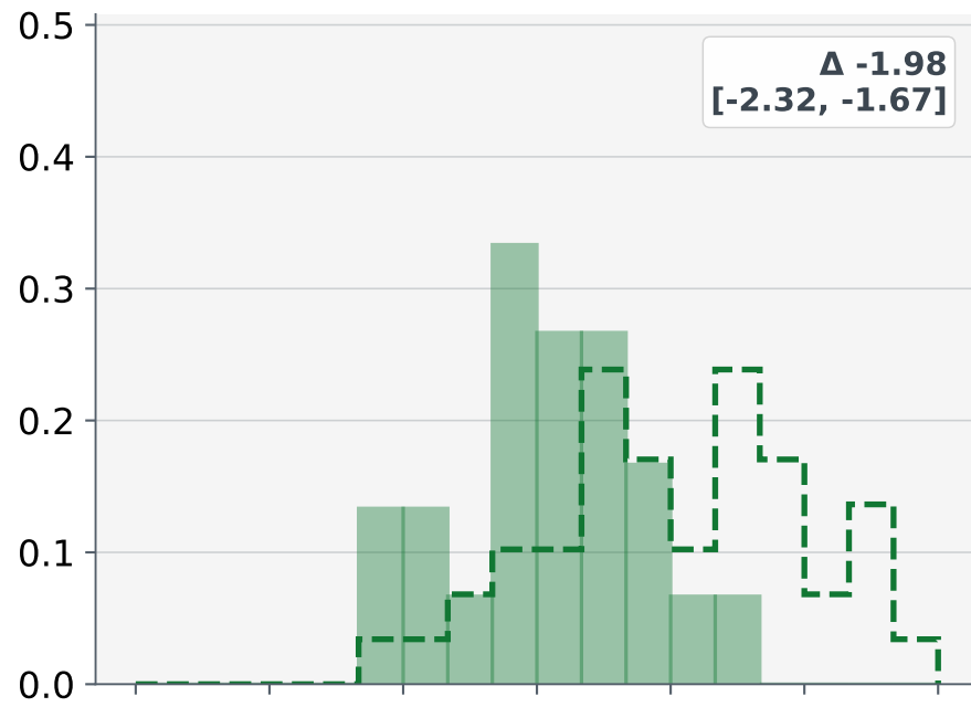
DeepSeek-V4 Flash
