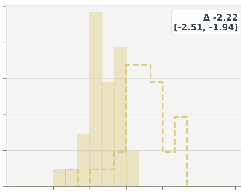
Mistral Small 4
