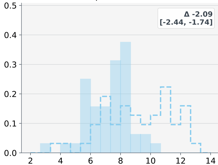
DeepSeek-V4 Flash
