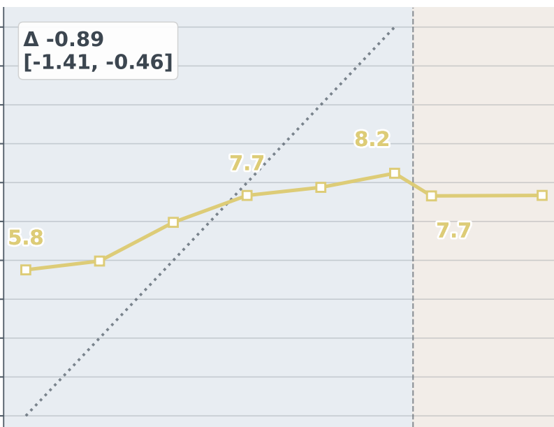
Claude Haiku 4.5
