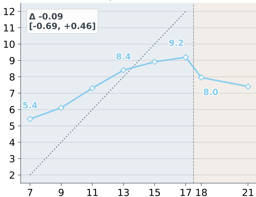
DeepSeek-V4 Flash
