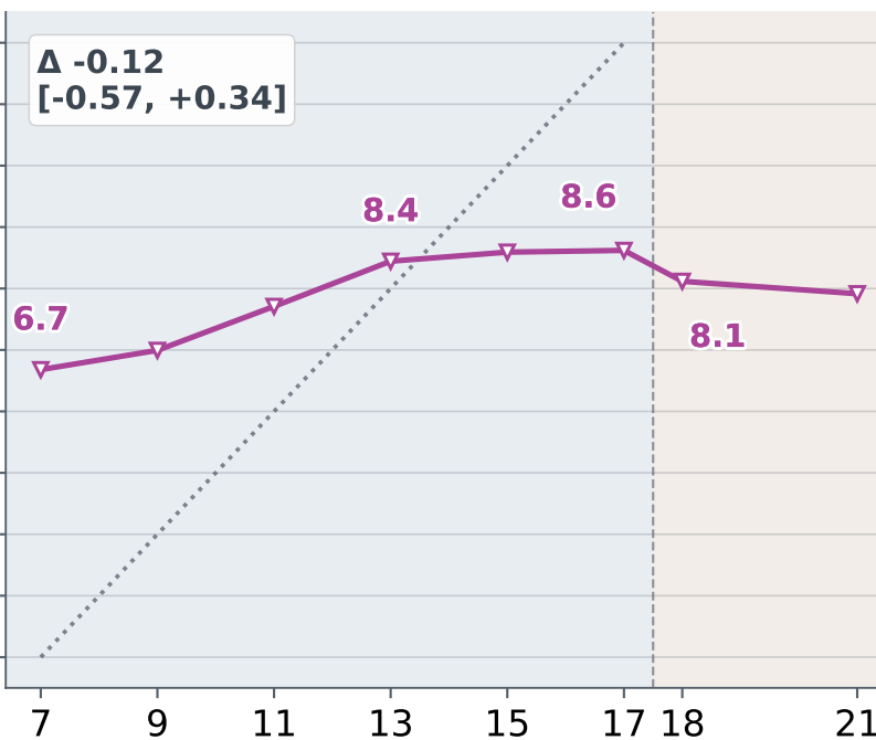
Mistral Small 4
