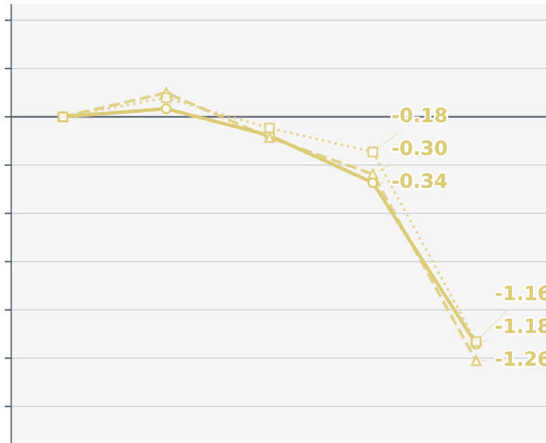
Mistral Small 4
