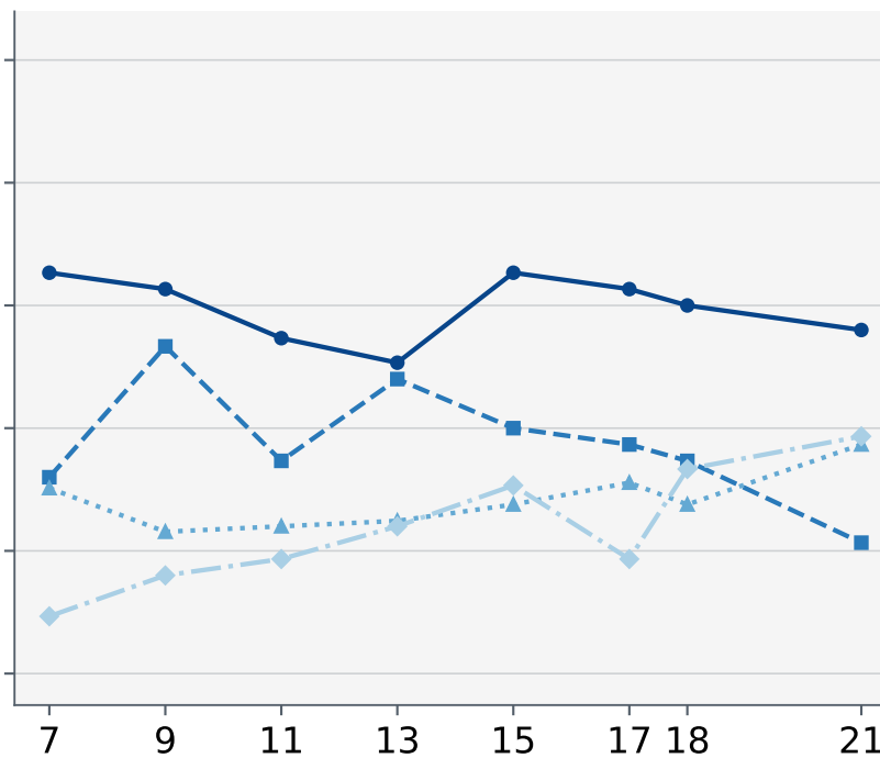
Mistral Small 4
