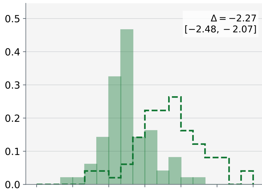
DeepSeek-V4 Flash
