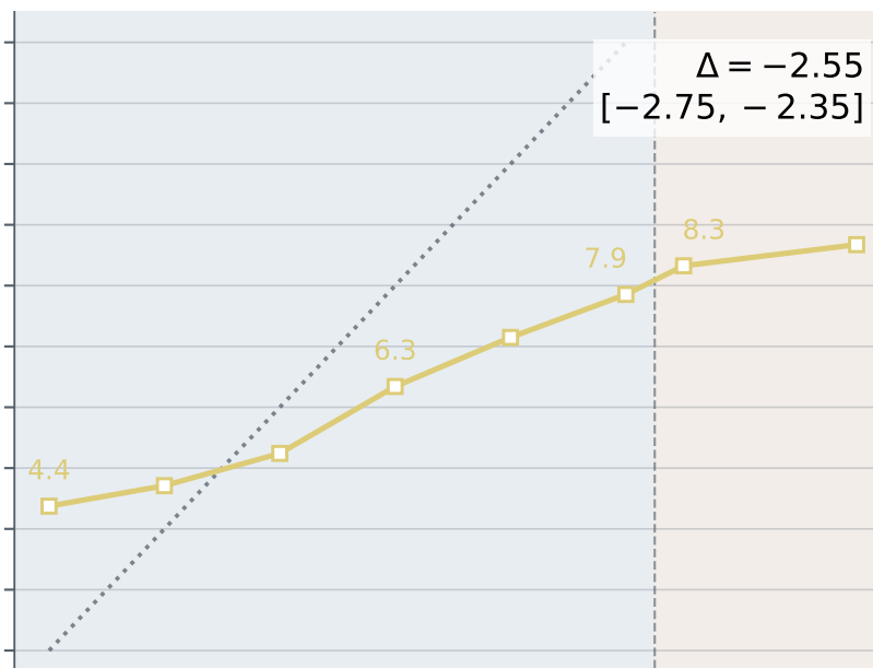
Mistral Small 4
