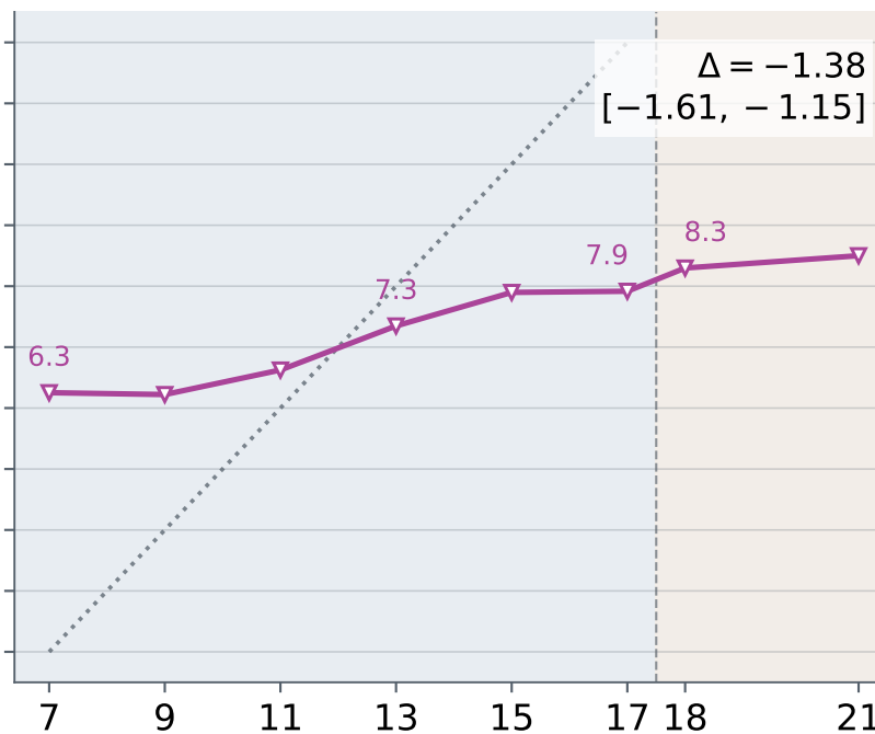
Mistral Small 4
