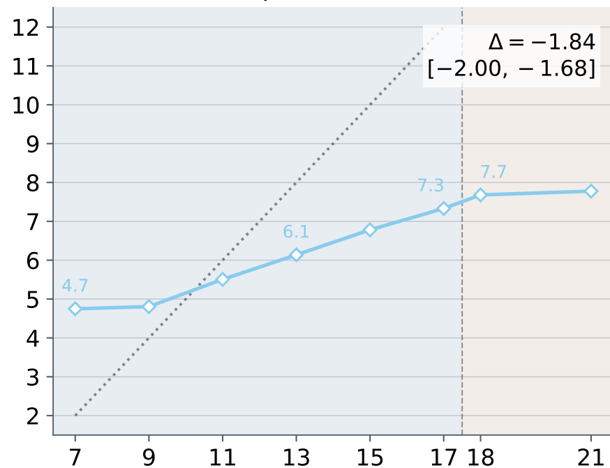
DeepSeek-V4 Flash
