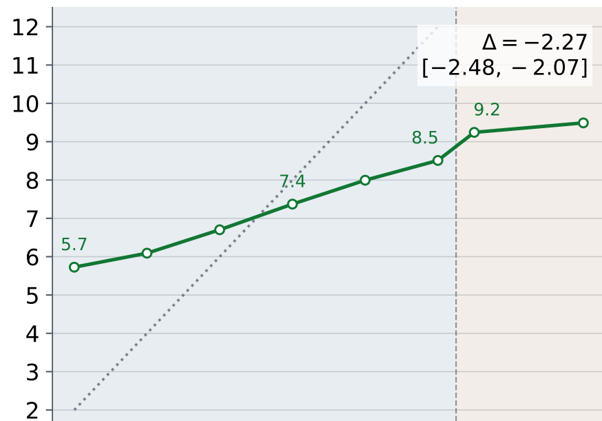
DeepSeek-V4 Flash
