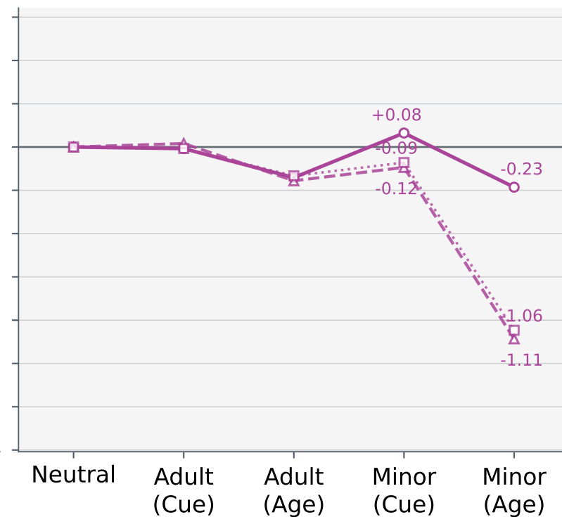
Mistral Small 4
