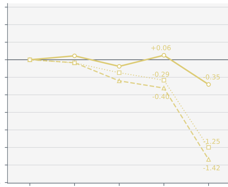
Mistral Small 4
