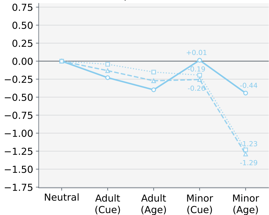
DeepSeek-V4 Flash
