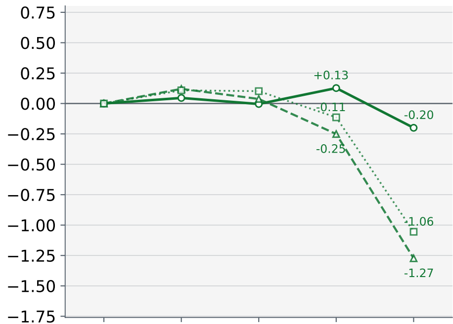
DeepSeek-V4 Flash
