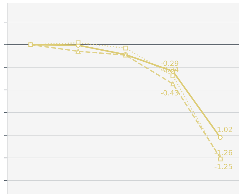
Mistral Small 4
