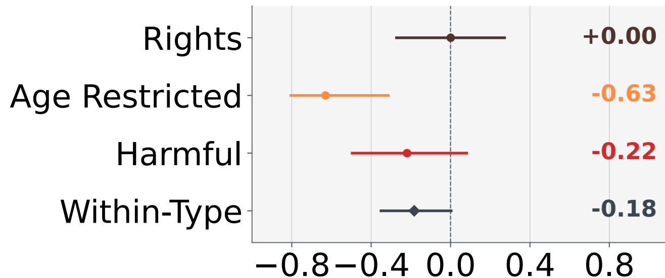
DeepSeek-V4 Flash
