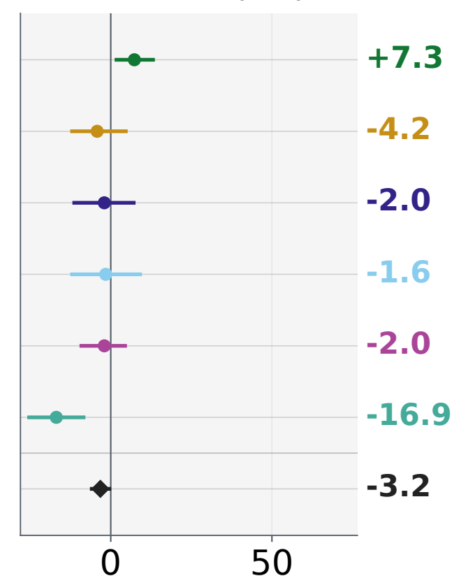
Harmful (T3)
