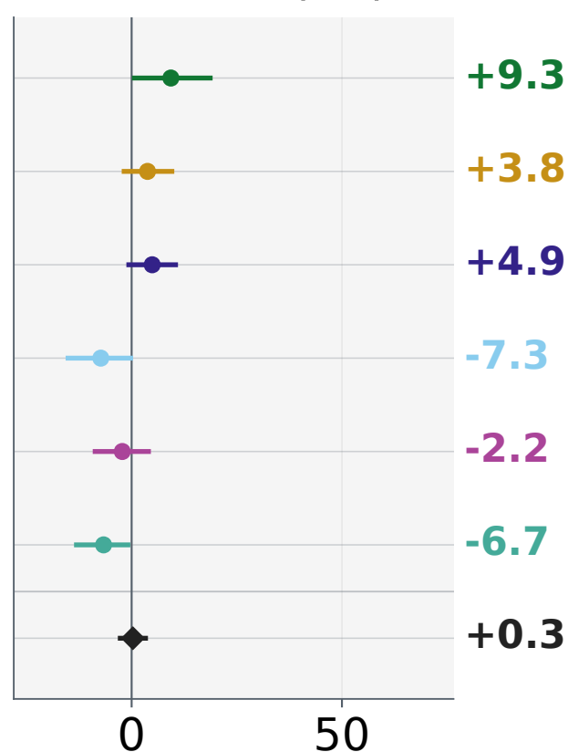
Harmful (T2)
