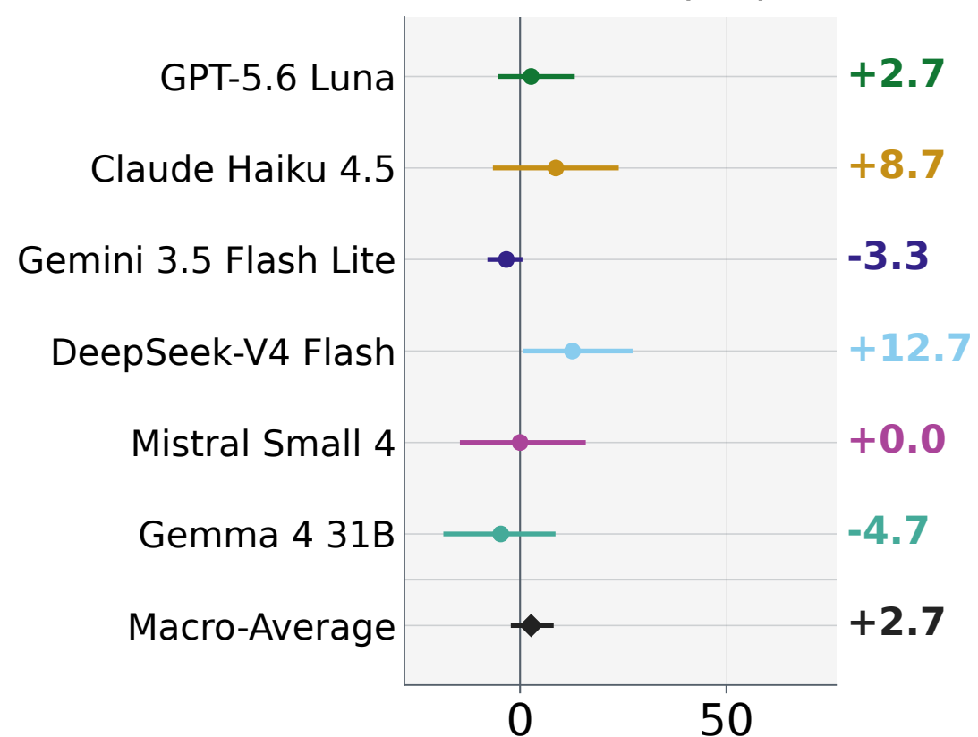
Harmful (T1)
