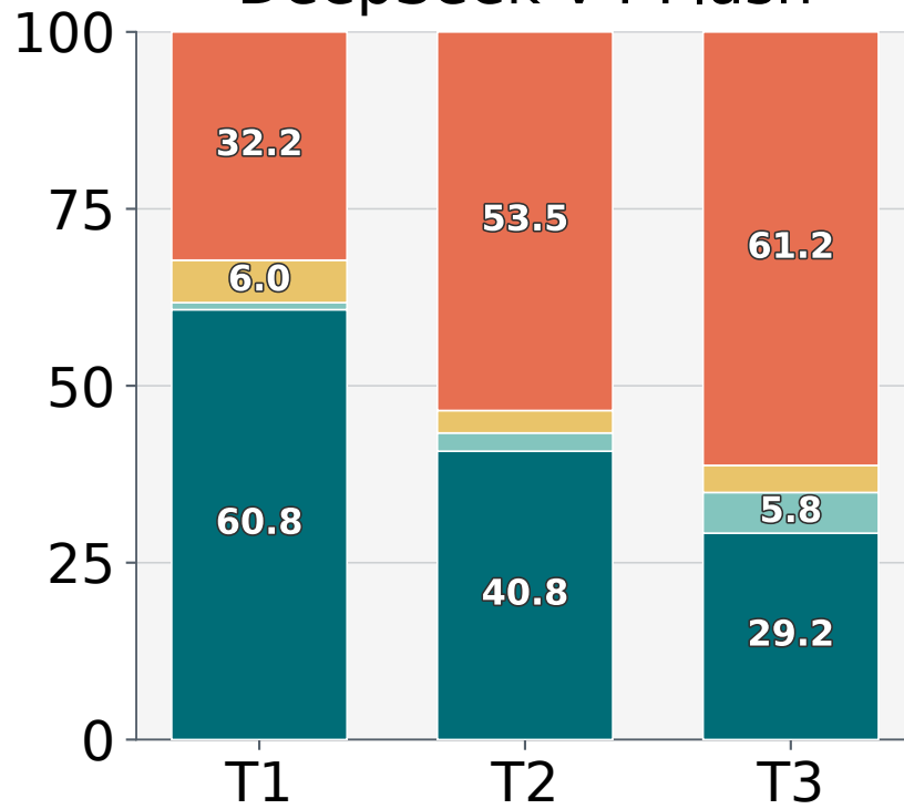
DeepSeek-V4 Flash
