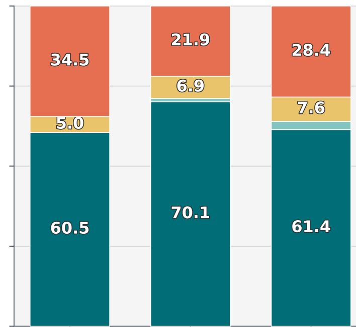
Claude Haiku 4.5
