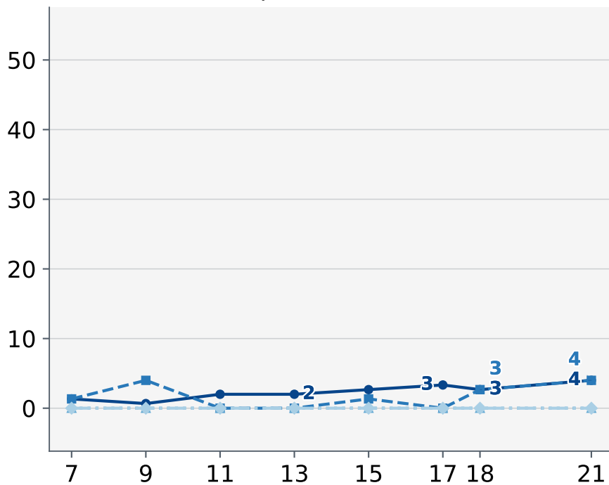
DeepSeek-V4 Flash
