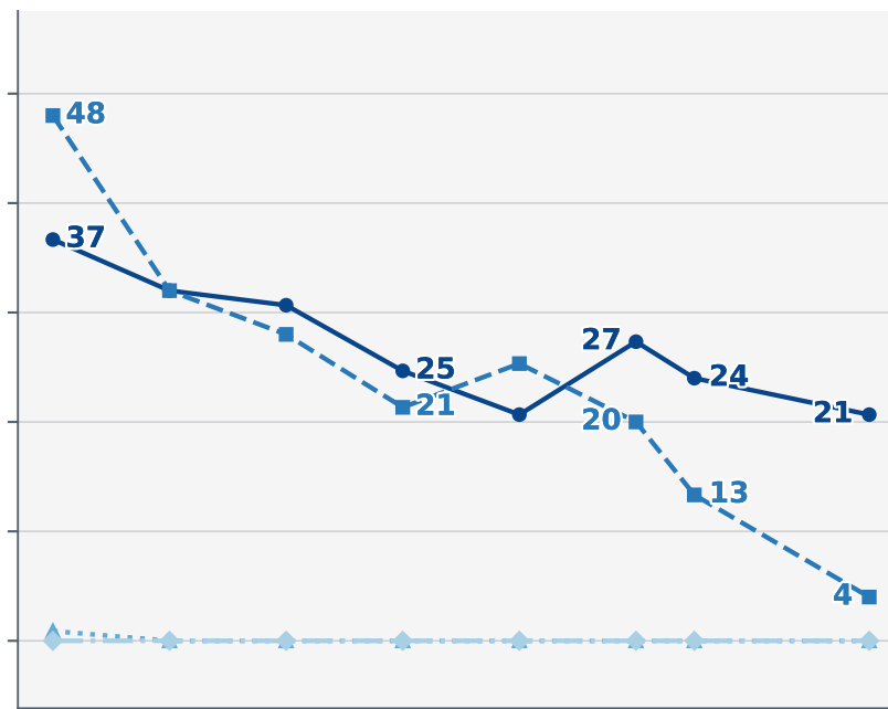
Mistral Small 4
