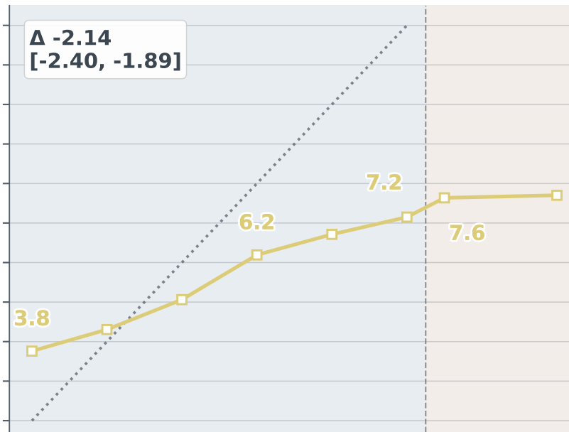
Mistral Small 4
